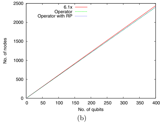
Fig. 9.10. (a) Runtime results for the matrix product, element-wise division, modulus and DD compare, and non-0 terminal merge algorithms to check for relative-phase equivalence in the Hamiltonian \Delta t circuit. (b) Node count as a function of the number of qubits.
