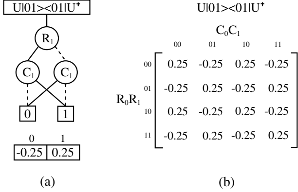
Fig. 8.1. (a) QuIDD for the density matrix resulting from U|01\rangle\langle 01|U^\dagger , where U = H \otimes H , and (b) its explicit matrix form.
