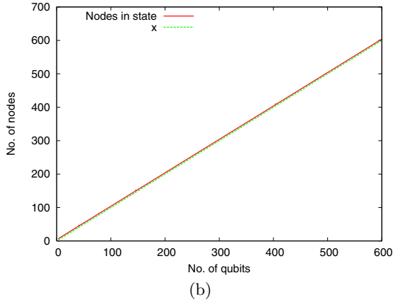
Fig. 9.4. (a) Runtime results for the inner product and GPRC on checking global-phase equivalence of states generated by a Grover iteration. (b) Node counts for the QuIDD representation of the state vector.
