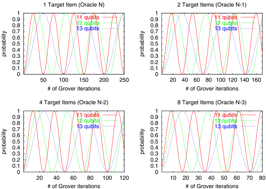
Fig. 7.5. Probability of successful search for 1, 2, 4 and 8 items as a function of the number of iterations after which the measurement is performed (11, 12 and 13 qubits).
