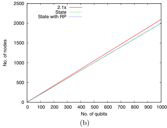
Fig. 9.8. (a) Runtime results for the inner product, element-wise division, modulus and DD compare, and non-0 terminal merge algorithms for checking relative-phase equivalence of the remote EPR pair circuit. (b) Node count as a function of the number of qubits.
