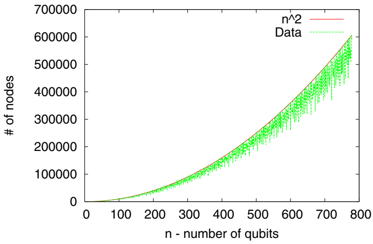
Fig. 7.14. Growth of inverse quantum Fourier transform matrix in QuIDD form.
